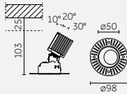
Trimless flange (Included)
