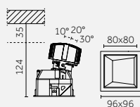
Visible trim flange (Included)
