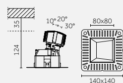
Trimless flange (Included)
