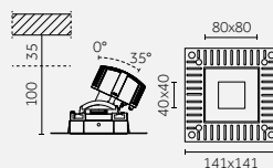
With trimless flange (To be ordered separately)
