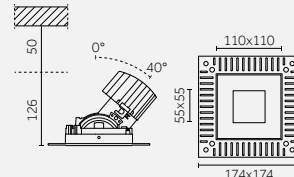
With trimless flange (To be ordered separately)
