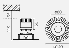
With trimless flange (To be ordered separately)
