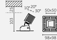
Trimless flange (Included)
