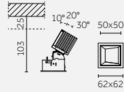
Visible trim flange (Included)
