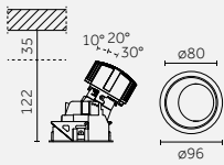
Visible trim flange (Included)
