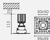
With trimless flange (To be ordered separately)
