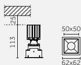
With visible trim flange (To be ordered separately)
